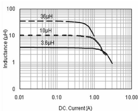
PWPI 4012 TYPE
