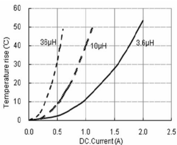
PWPI 4012 TYPE
