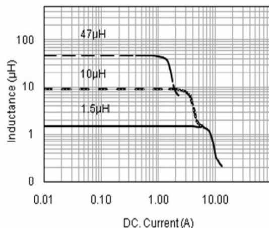
PWPI 5040 TYPE
