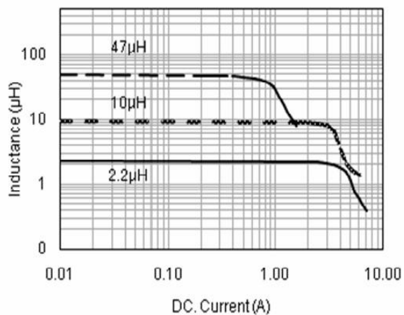
PWPI 5020 TYPE
