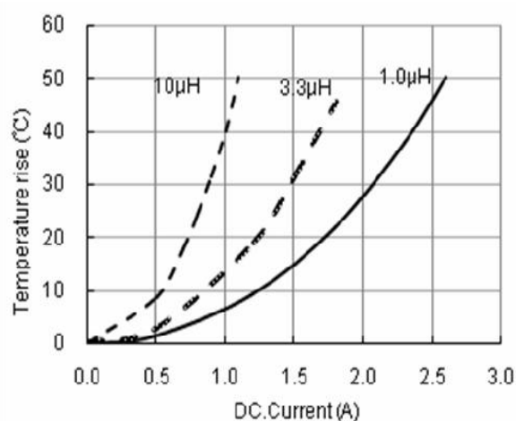
PWPI 5012 TYPE
