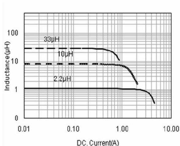
PWPI 4026 TYPE
