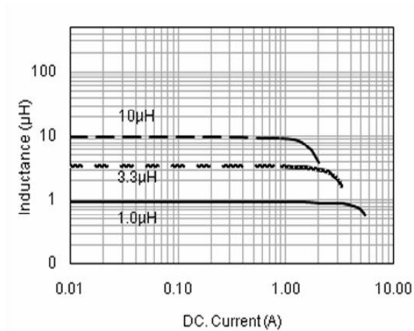
PWPI 5012 TYPE
