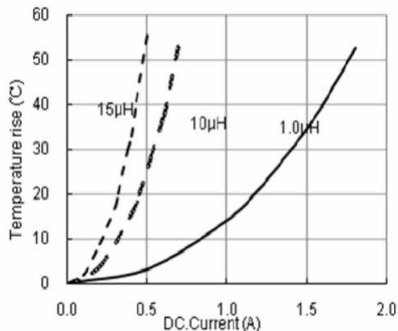
PWPI 252012 TYPE
