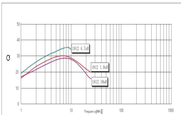
PWFI 4532(1812) TYPE
