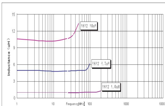
PWFI 4532(1812) TYPE
