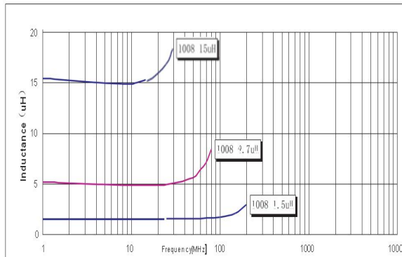
PWFI 2520(1008) TYPE
