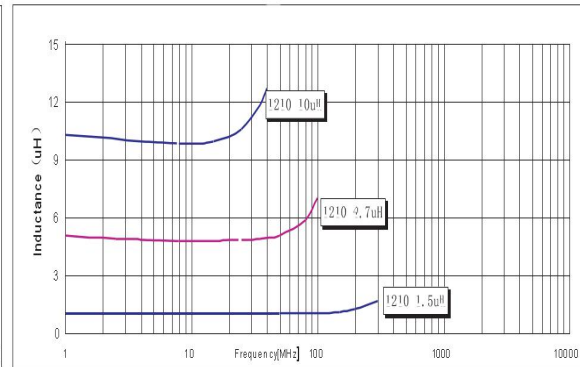
PWFI 3225(1210) TYPE
