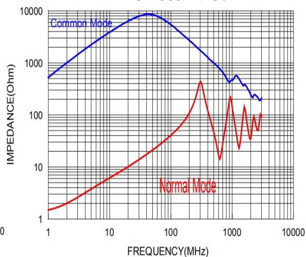
PICM3532N750T2L
