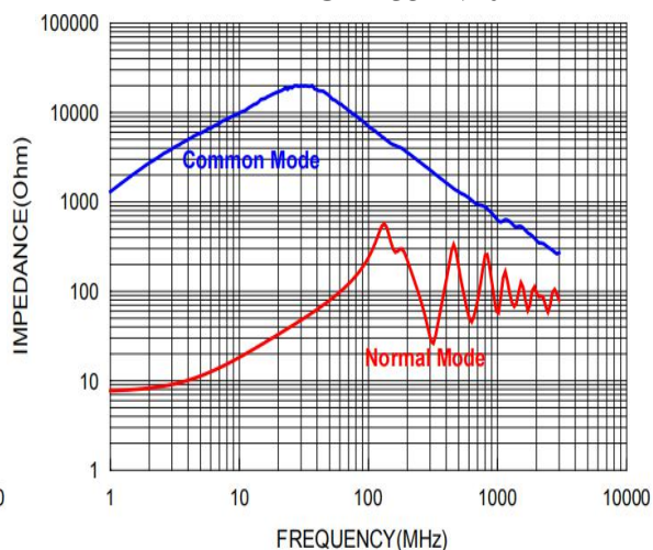
PICM4532N201T2L
