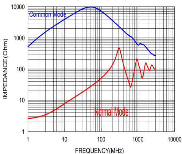
PICM3225N101T2L
